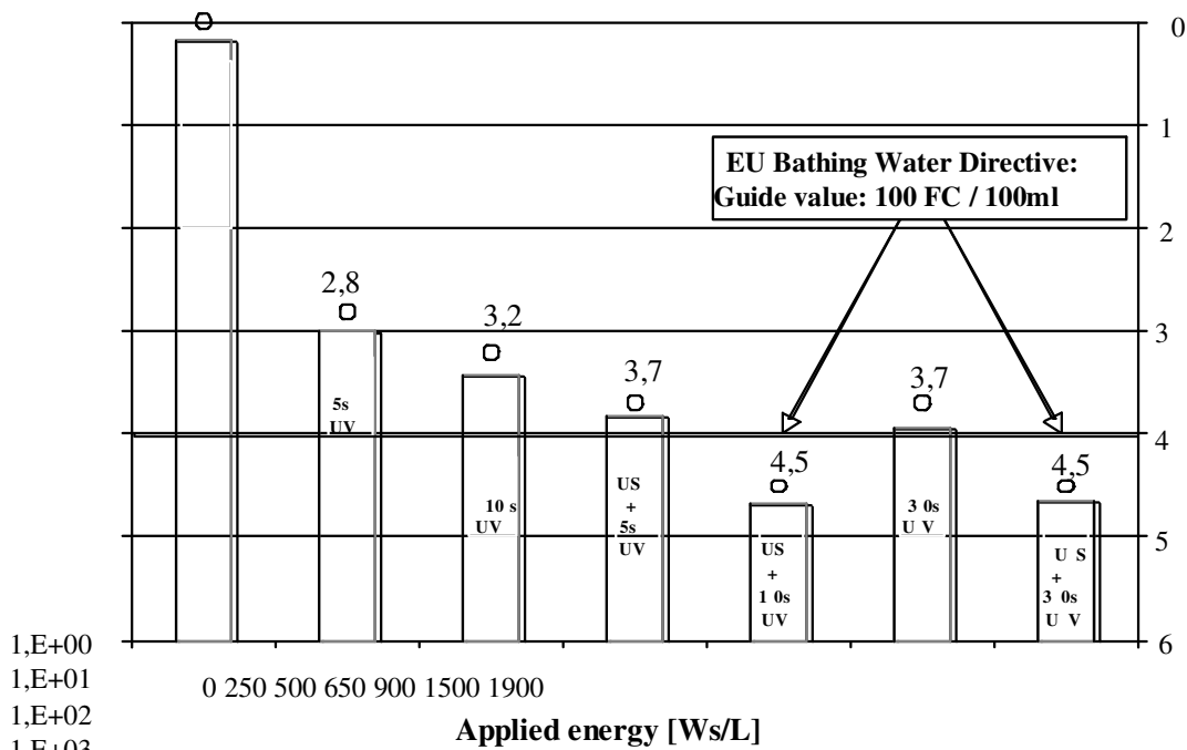
Figure 5: Improved UV disinfection (density: 50 W/L) by ultrasonic pre-treatment (sonication time: 5 s, density: 80 W/L) to meet the Bathing Water guide value (abscissa not to scale)
