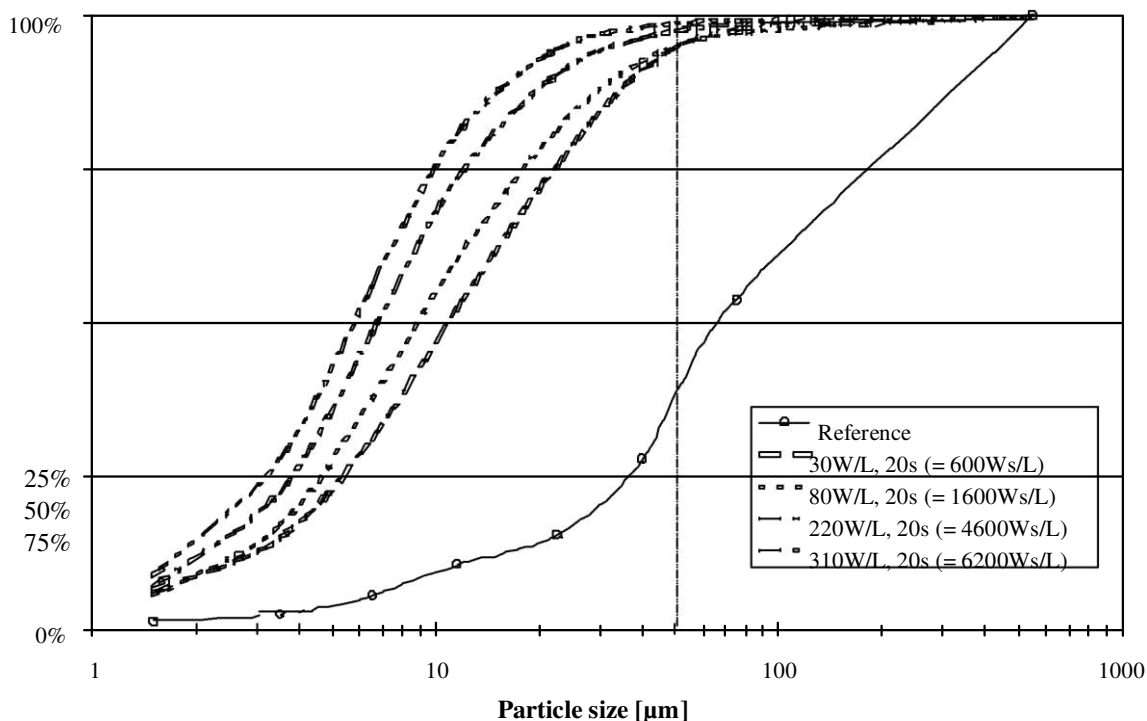
Figure 2: Effect of wastewater sonication (20 s at various densities) on PSD
