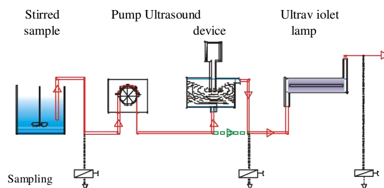
Figure 1: Flow scheme of the experimental set-up
