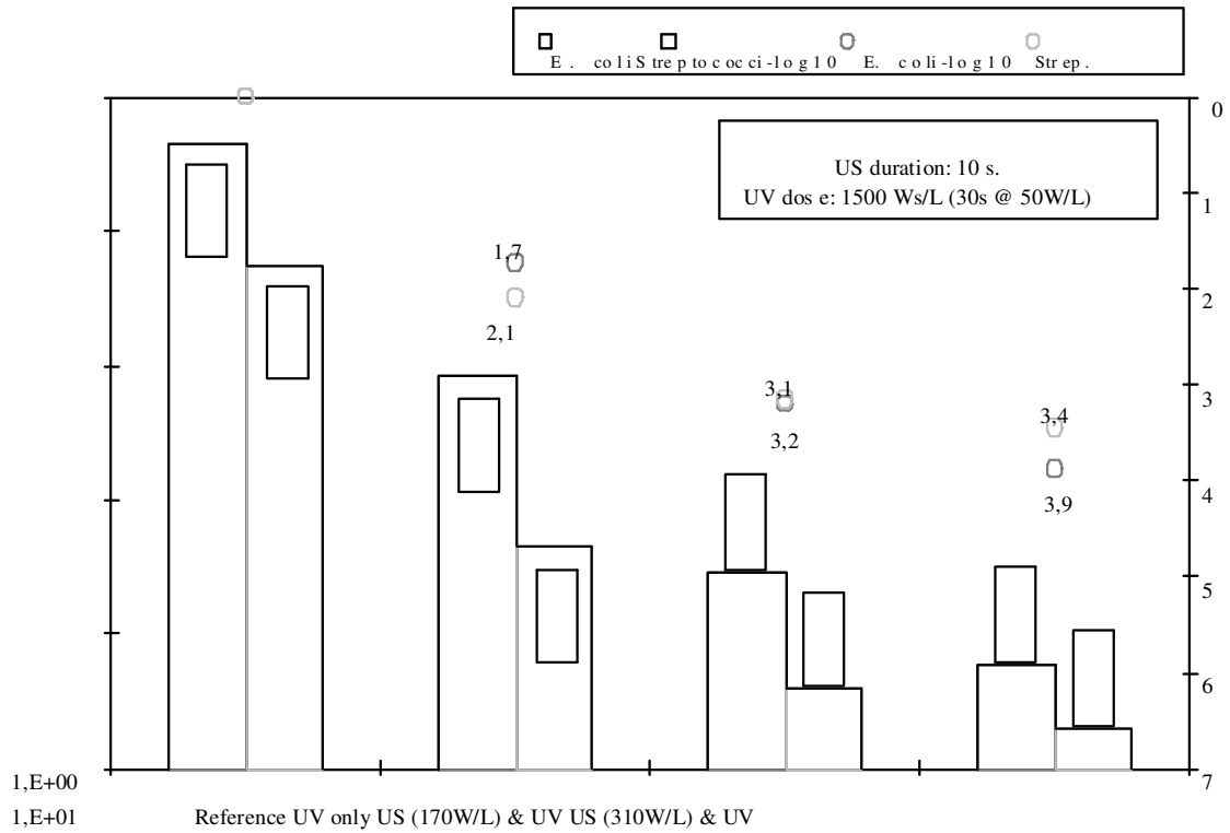
Figure 4: Reduction of E. coli and fecal streptococci by ultrasonic pre-treatment for 10 s followed by UV irradiation for 30 s
